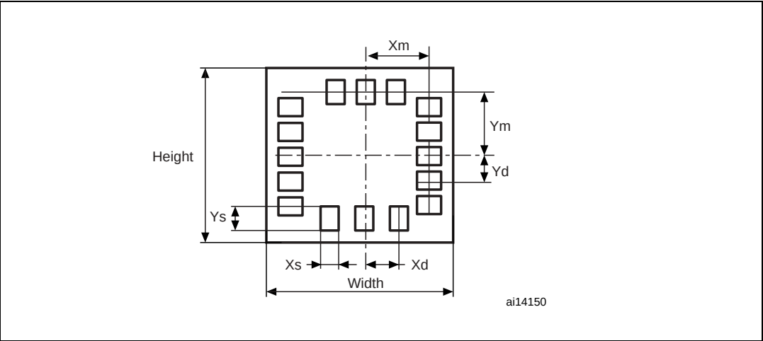
Figure 7. MEMS footprint (LAG16 (A) package)
