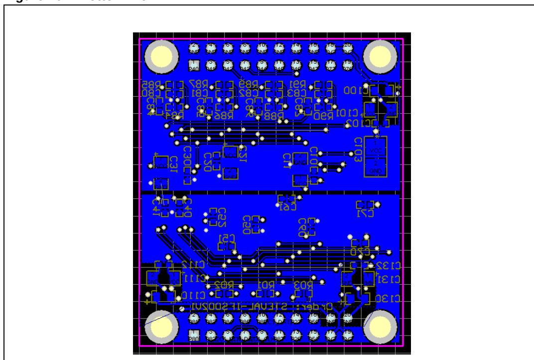
Figure 10. Bottom view
